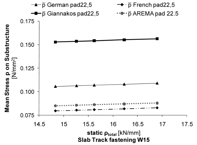
Fig. 10 Mean stress on substructure in the case of ballastless (Slab) track equipped with W15 Fastening with pad Zw104 ( \rho_{\text{pad}}=22.5 \text{ kN/mm} or 128.5 \text{ kips/in} ) in relation to the static total track stiffness total according to the methods cited in the German, French, American Literature and Giannakos (2004) method.
