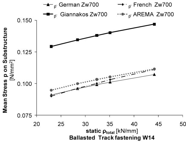
Fig. 9 Mean stress on substructure in the case of classic ballasted track equipped with W14 Fastening with pad Zw700 ( \rho_{\text{pad}}=50 \text{ kN/mm} ) in relation to the static total track stiffness \rho_{\text{total}} according to the methods cited in the German, French, American Literature and Giannakos (2004) method.
