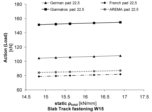
Fig. 6 Actions on the track panel as a function of the static total track stiffness \rho_{\text{total}} for the case of ballastless track equipped with W15 fastening and Zw104 pad ( \rho_{\text{pad}} = 22.5 kN/mm).
