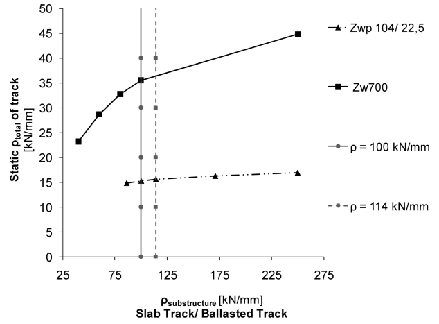
Fig. 4 Relation between static stiffness coefficient of substructure substruct and total static stiffness coefficient total in ballasted and ballastless (slab) track, for resilient fastening (W14 and pad Zw700) with \rho_{pad} \approx 50 \text{ kN/mm} in the ballasted track case and W15 fastening (with pad Zw104) with \rho_{pad} \approx 22.5 \text{ kN/mm} in the slab track case.
