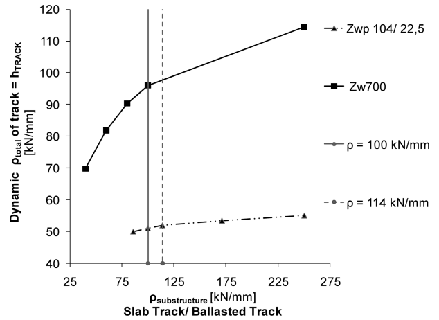
Fig. 5 Relation between static stiffness coefficient of substructure substruct and total dynamic stiffness coefficient h_{TRACK} in ballasted and ballastless (slab) track, for resilient fastening (W14 and pad Zw700) with \rho_{pad} \approx 50 \text{ kN/mm} in the ballasted track case and W15 fastening (with pad Zw104) with \rho_{pad} \approx 22.5 \text{ kN/mm} in the slab track case.
