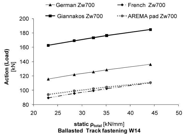
Fig. 7 Actions on the track panel as a function of the static total track stiffness \rho_{\text{total}} for the case of classic ballasted track equipped with W14 fastening and Zw700 pad ( \rho_{\text{pad}} = 50 kN/mm).
